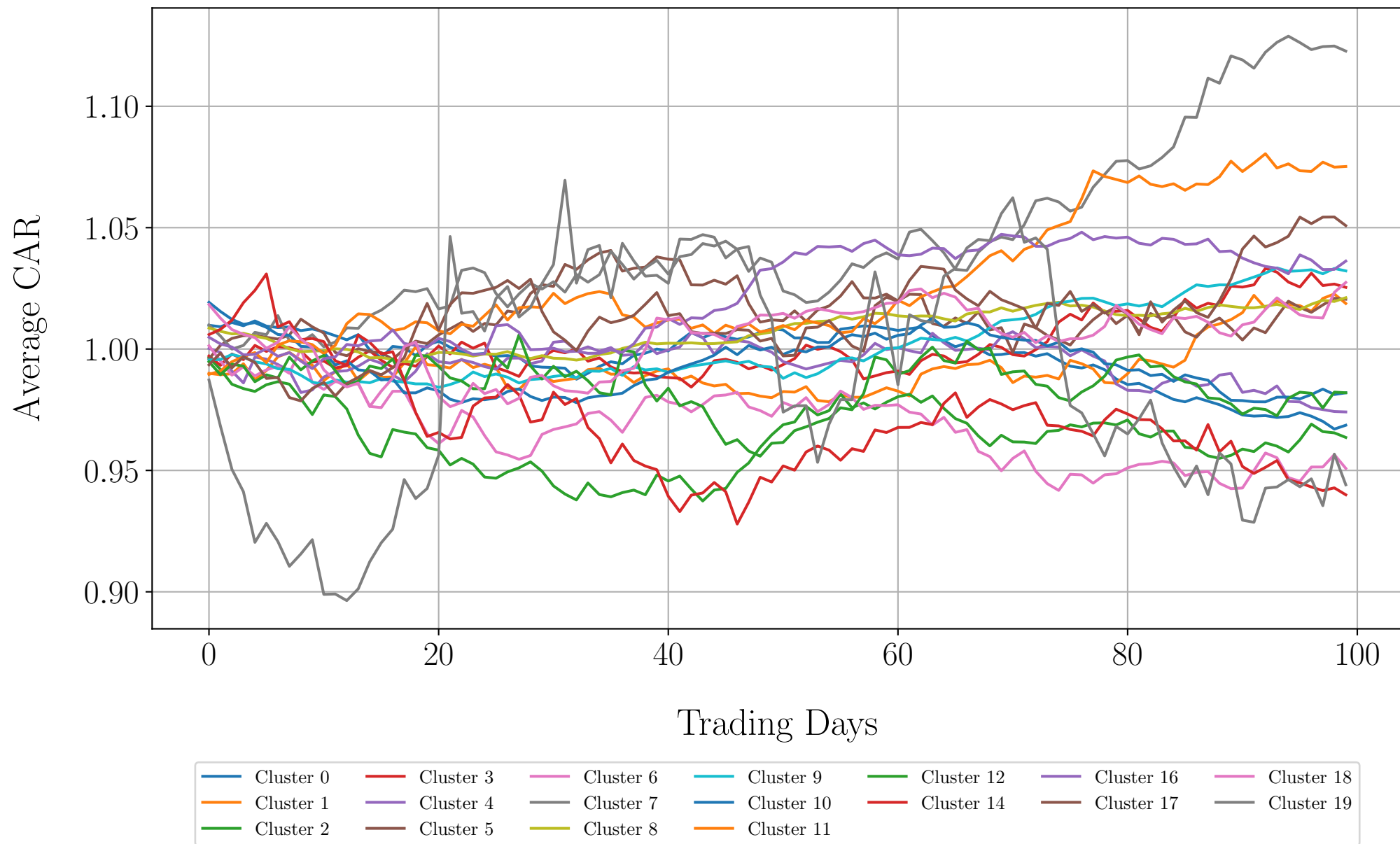
Average CARs for each cluster (Train)
